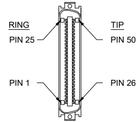
RJ21 CAT5 MALE CONNECTOR (CAT3 AVAILABLE)
