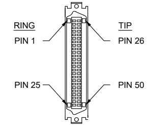
RJ21 CAT5 FEMALE CONNECTOR (CAT3 AVAILABLE)
